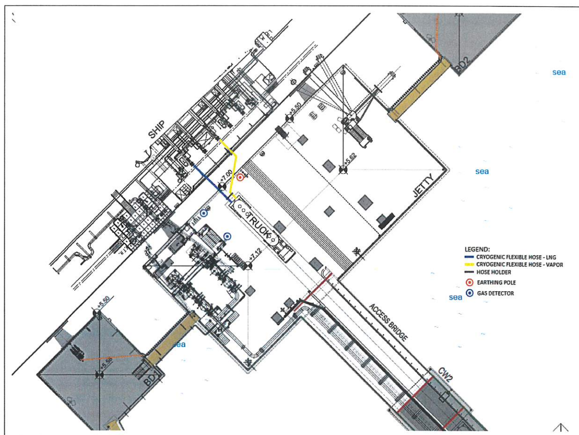
Figure 1.1 Ship-To-Truck visualization
